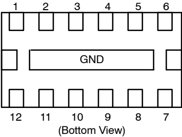
Figure 3. Pin Diagram
