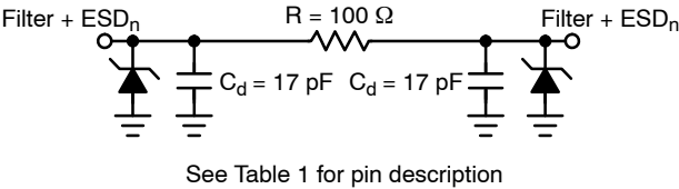
Figure 1. Electrical Schematic
