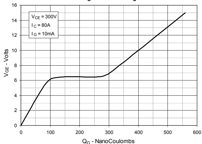
Fig. 7. Gate Charge
