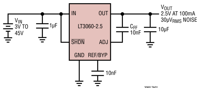
2.5V Low Noise Regulator
