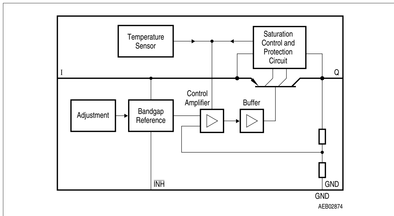
Figure 1 Block diagram
