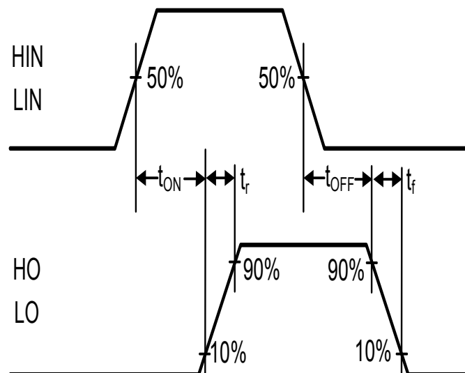
Figure 3. Input-to-Output Delay Timing Diagram
