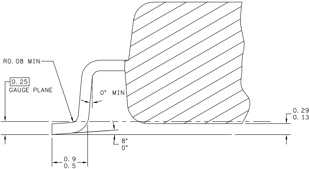
SECTION B-B
