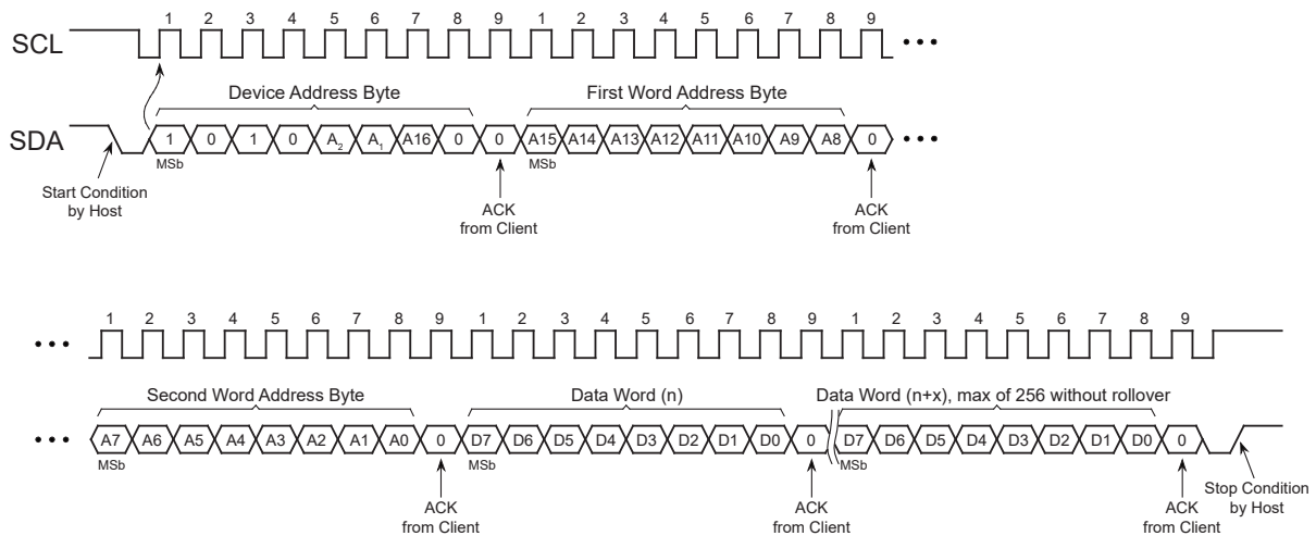
Figure 7-2. Page Write
