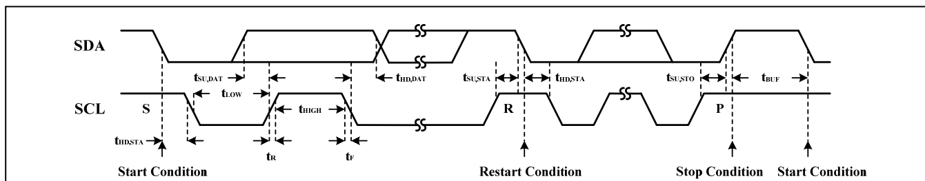
Figure 3 Interface Timing
