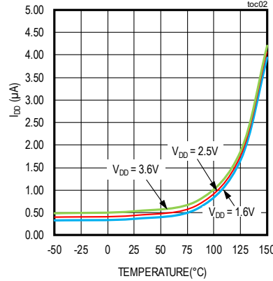
SUPPLY CURRENT vs. TEMPERATURE (SHUTDOWN MODE WITH TIMEOUT DISABLED)
