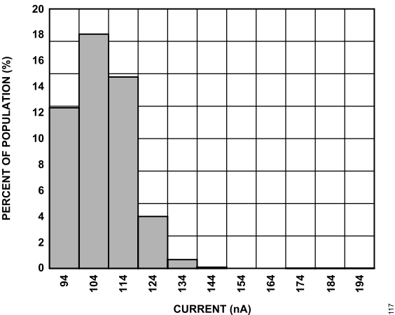
Figure 18. Standby Mode Current Consumption at 25°C, V_S = 2.5\text{ V}
