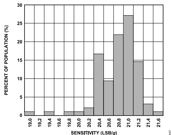
Figure 8. Y-Axis Sensitivity Deviation at 25°C, V_S = 2.5 V
