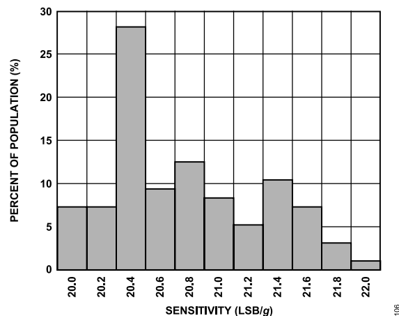
Figure 7. X-Axis Sensitivity Deviation at 25°C, V_S = 2.5 V
