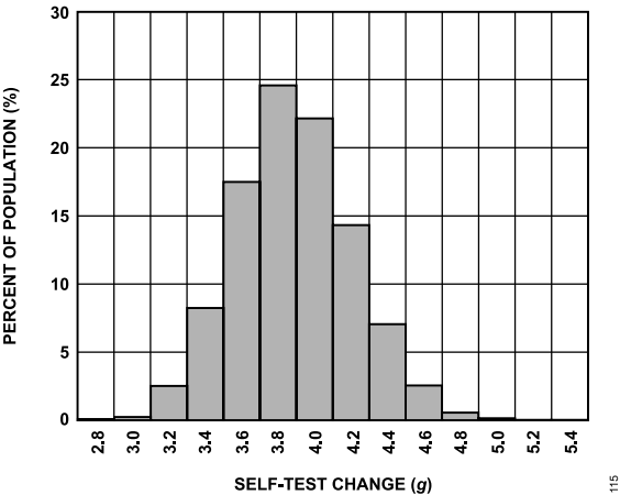
Figure 16. Z-Axis Self Test Response at 25°C, V_S = 2.5\text{ V}
