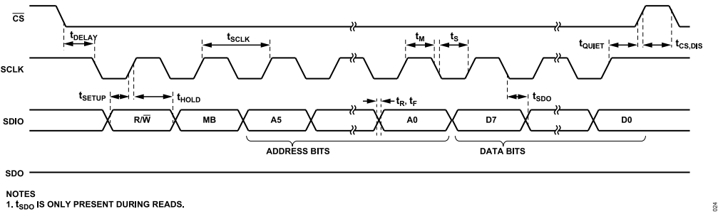
Figure 25. SPI 3-Wire Read and Write
