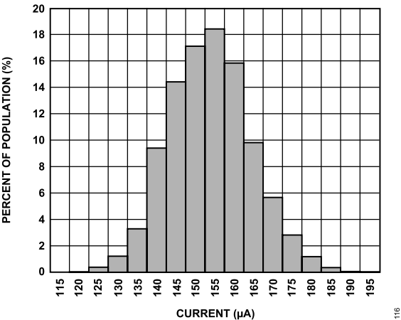
Figure 17. Measurement Mode Current Consumption at 25°C, V_S = 2.5\text{ V}
