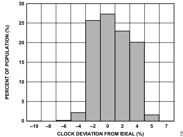
Figure 19. Clock Frequency Deviation from Ideal at 25°C, V_S = 2.5\text{ V}
