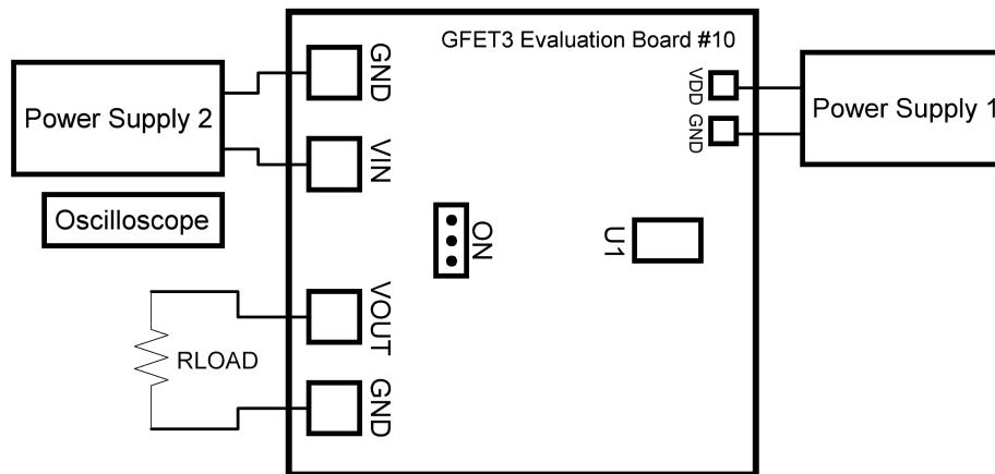
Figure 6. Typical connections for GreenFET Evaluation.
