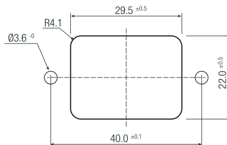
Mounting hole dimensions
