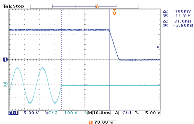
Figure 5 ECP150PS12 100VAC 100W load
