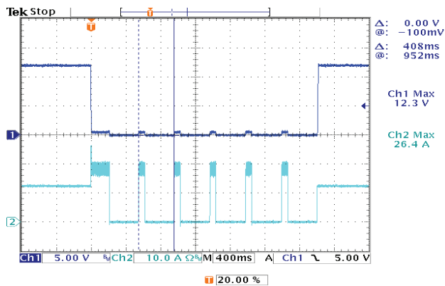
Figure 2 ECP150PS12
