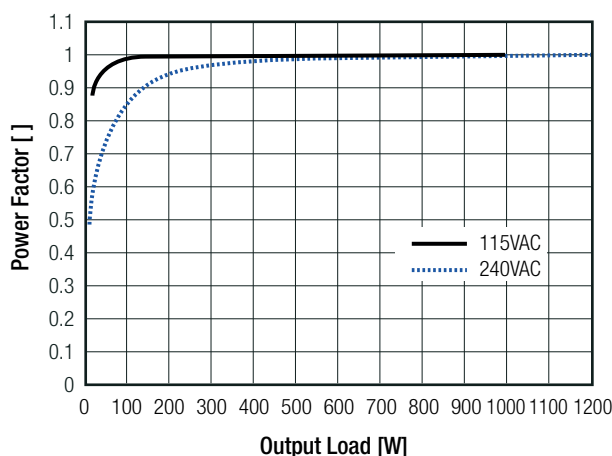
Power Factor
