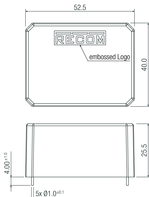
Dimension Drawing THT-printmount version SINGLE and DUAL Output (mm)
