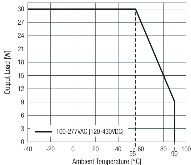
RACM30-xxSK/277/OF others
