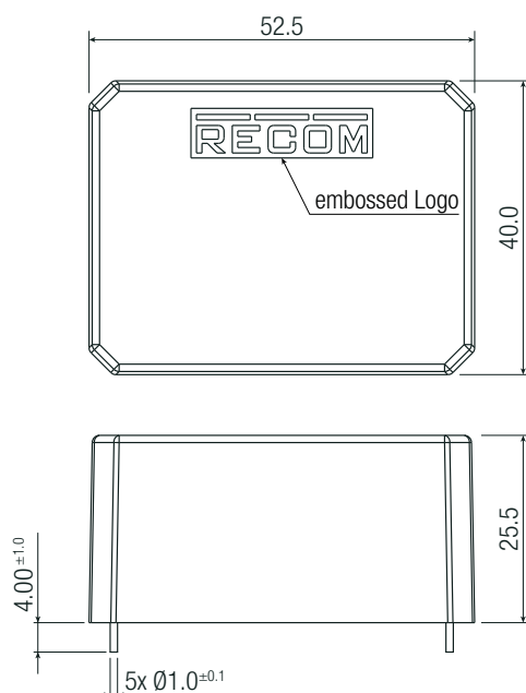
Dimension Drawing THT-printmount version SINGLE and DUAL Output (mm)
