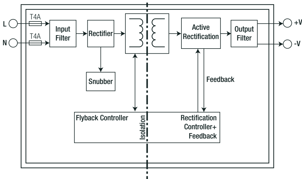
Blockdiagram (“/ENC”)
